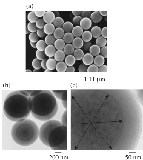
Figure 2. (a) SEM image of the core/shell MMSS. (b) and (c) TEM images of the platinum-introduced silica/mercaptopyrlyl-modified silica core/shell MMSS. Pore directions are shown by arrows.
